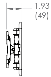
MOUNTING PROFILE
